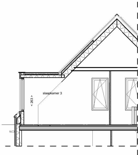
code 10500: dakkapel
