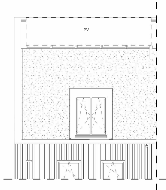
code 10500: dakkapel
