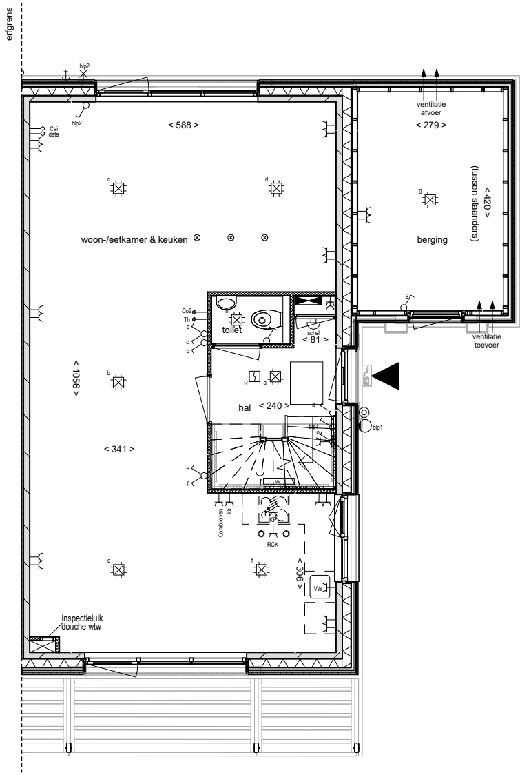
00 begane grond
