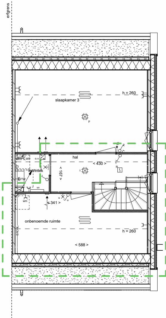
zolder
